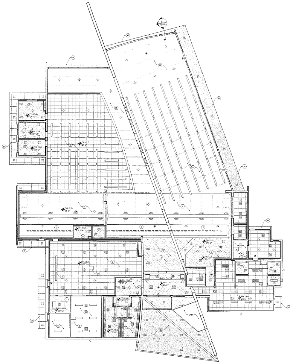
(A1) MAIN LEVEL REFLECTED CEILING PLAN REVIT.DWG
