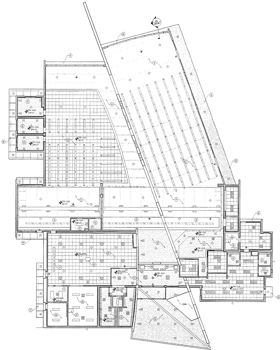
(A) MAIN LEVEL REFLECTED CEILING PLAN
